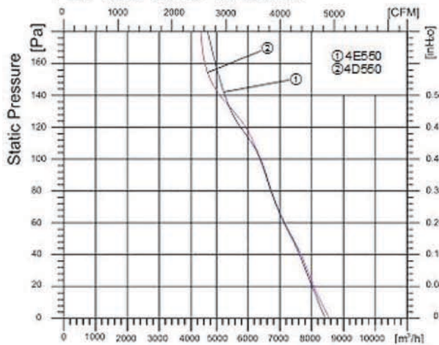
Flow Rate Curve-4E/4D/550
